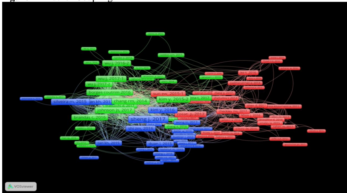
Figure 1 - Author Coupling
