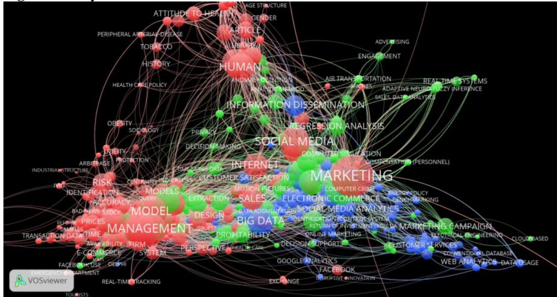
Figure 2 - Keywords Co-occurrence
