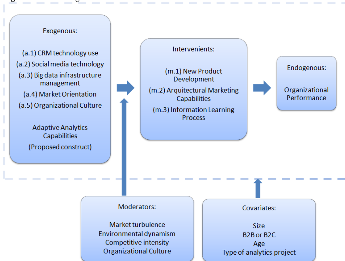
Figure 4 - Nomological network
